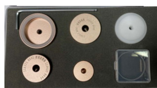
ST-5445-Die set use to replace crystals & gaskets for RLX. Made for 116400 BK41
