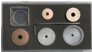
ST-5443-Die set use to replace crystals & gaskets for RLX. Made for 116710-TC 30.4 BK40
